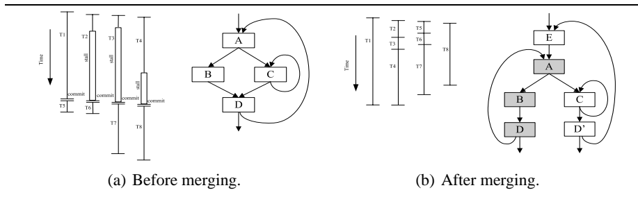
Fig. 4. Iteration merging.
