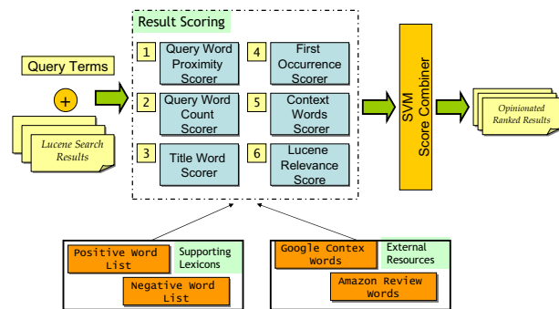
Figure 4: After relevant posts are retrieved, they are scored by various heuristics and an overall measure of opinionatedness computed by a SVM.
