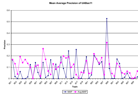
Figure 8: Mean average precision of submission UABas11
