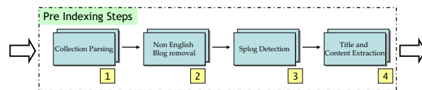
Figure 3: BlogVox text Preparation steps: (i) parsing the TREC corpus (ii) removing non English posts (iii) Eliminating splogs from the collection (iv) removing spurious material from the DOM tree.
